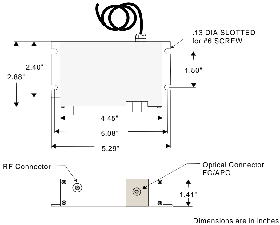
Figure 3-2 Flange-mount package dimensions.
