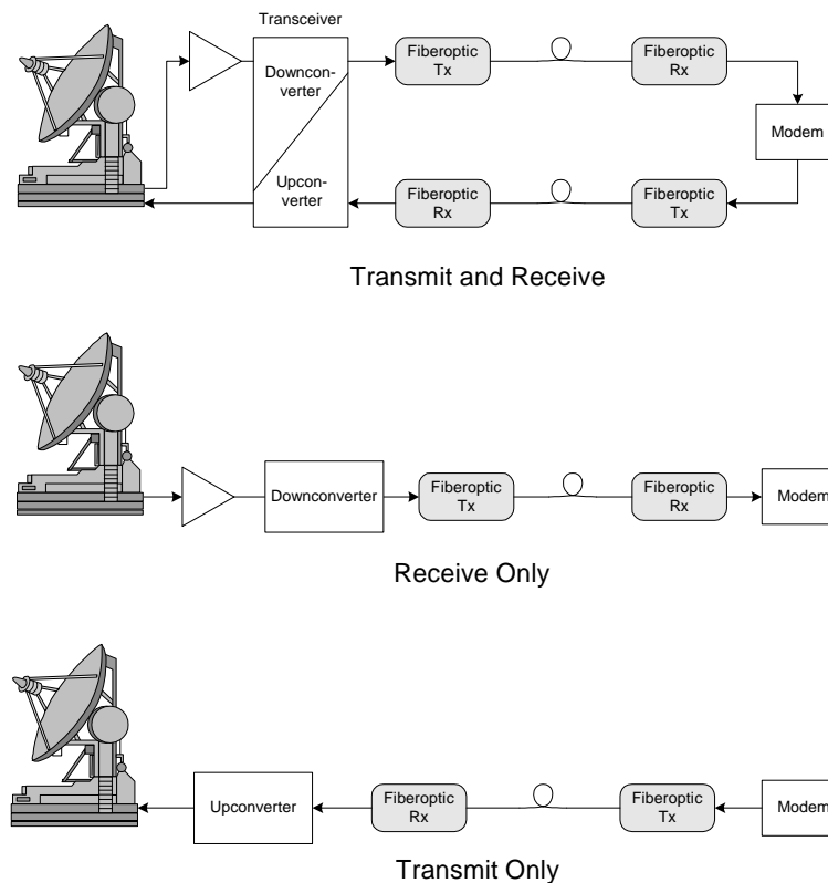
Figure 1-1 Typical applications of the Ortel IF-band IFL.
