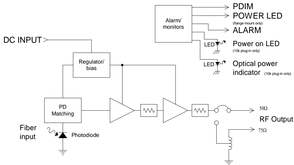
Figure 1-4 IF-band receiver block diagram. High gain (option 102) configuration is shown. Standard gain model has a single stage pre-amplifier.
