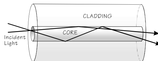
Figure 4-1 Light propagation in a step indexed fiber
