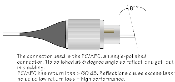
Figure 4-2 FC/APC style optical connector.
