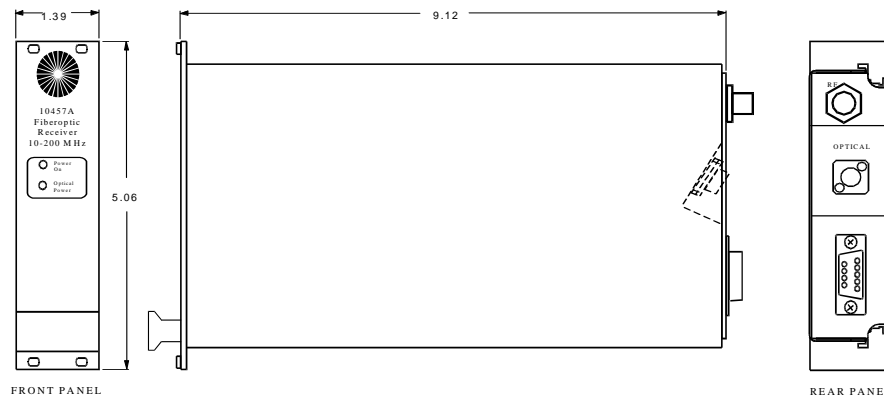
Figure 3-3 Plug-in package dimensions.
