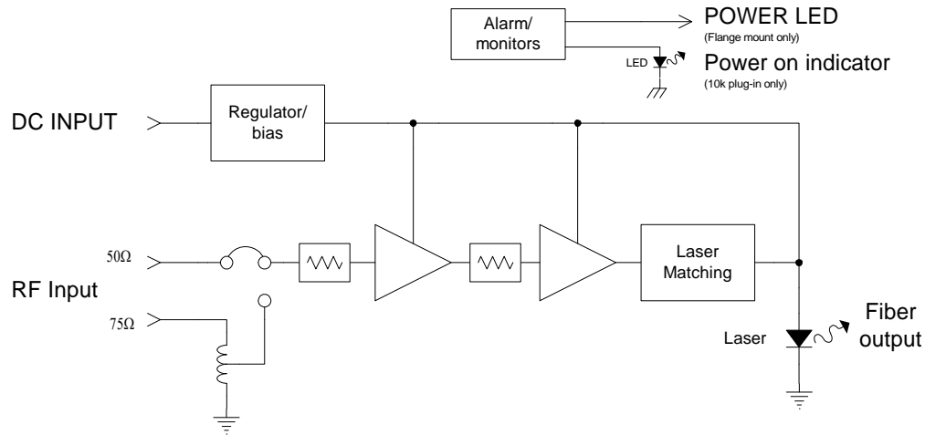
Figure 1-3 IF-band transmitter block diagram. Standard gain configuration is shown. Low gain model (option 102) has a single stage pre-amplifier.
