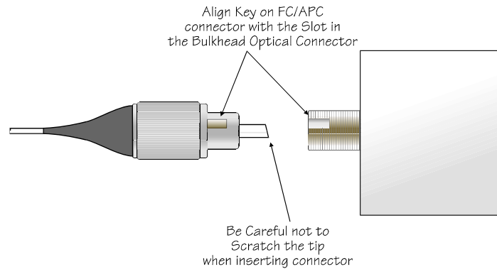
Figure 4-4 Inserting FC-APC connectors.
