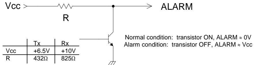
Figure 3-1 ALARM circuit for both flange-mount and plug-in style IF-band receivers. Transistor switches at approximately 0.1mW received optical power.
