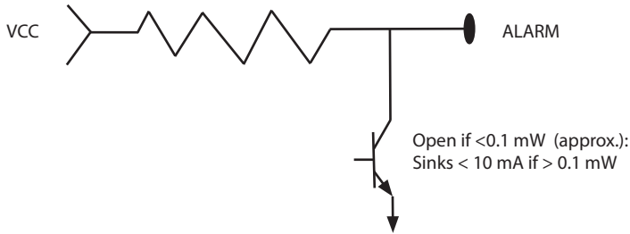
Figure 1. Receiver Electrical Schematic for Power Alarm
